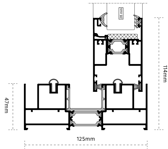
Double track (flush option)
