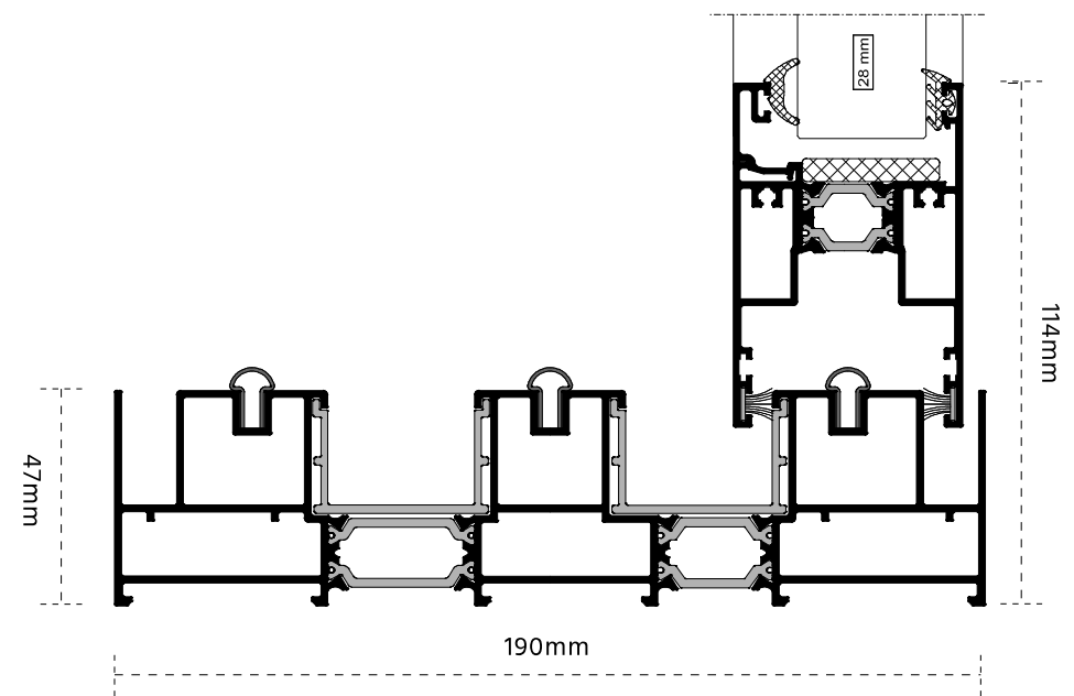
Triple track (flush option)
