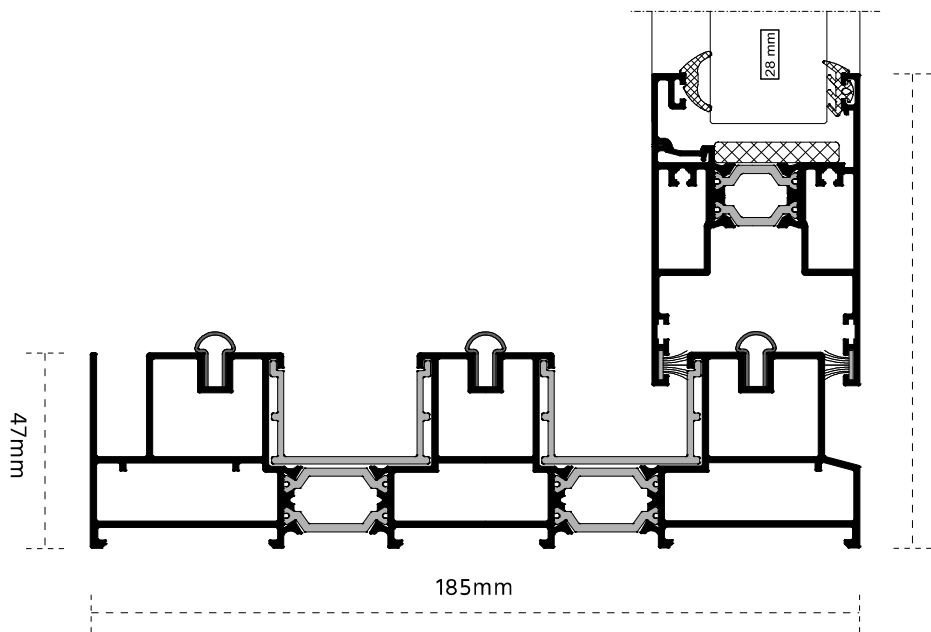
Triple track
