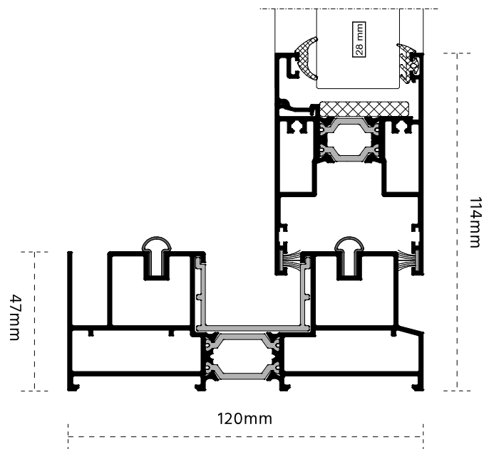
Double track
